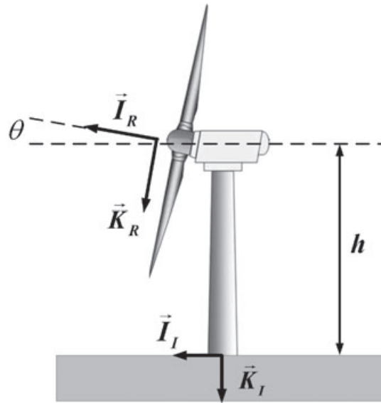
Figure 2. Turbine reference frame schematic.
